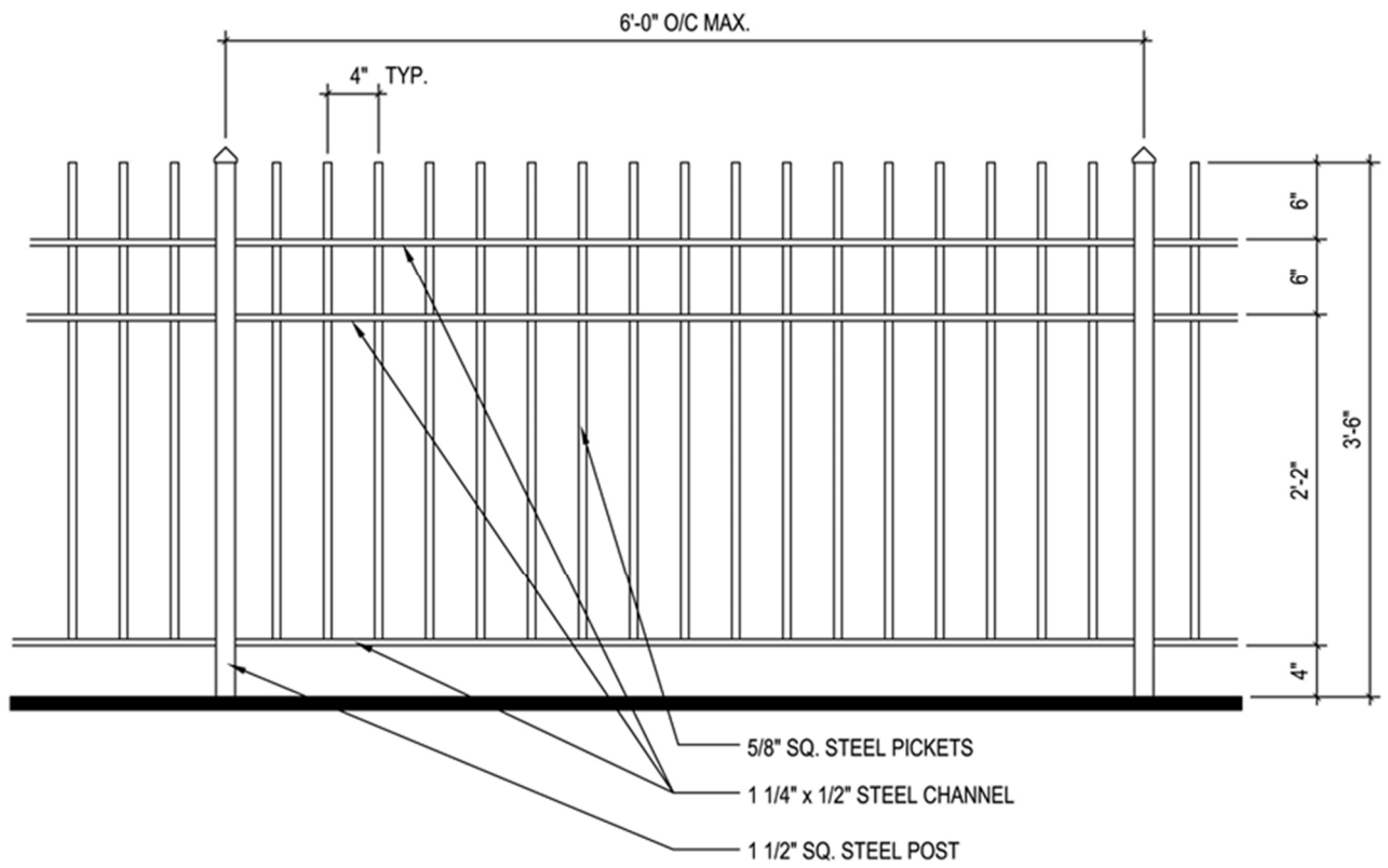
Figure C-28 – Metal Fences
