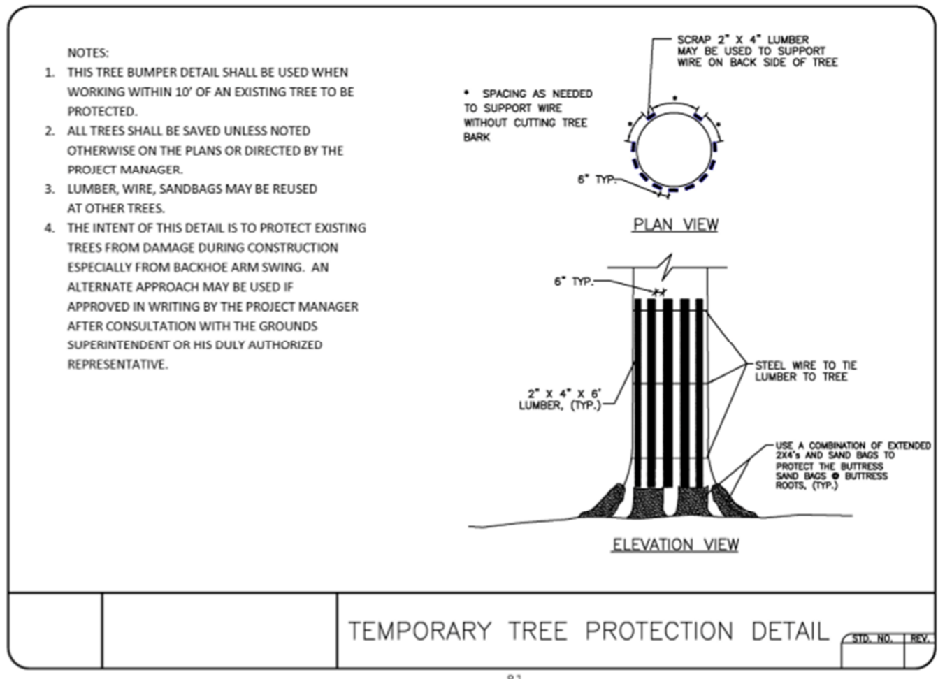
Figure C-39 – Temporary Tree Protection Detail
